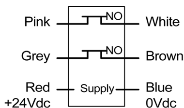
HE1 / HE2 Contacts 2NO (Note: Yellow & Green not connected)
