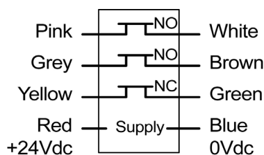
HE1 / HE2 / HE3 / HE6 / HED Contacts 2NO + 1 NC
