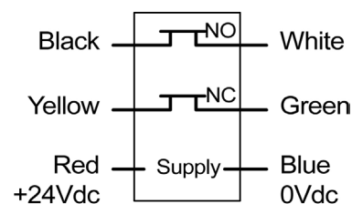
HE1 / HE2 Contacts 1NO + 1 NC (See Note 1)
